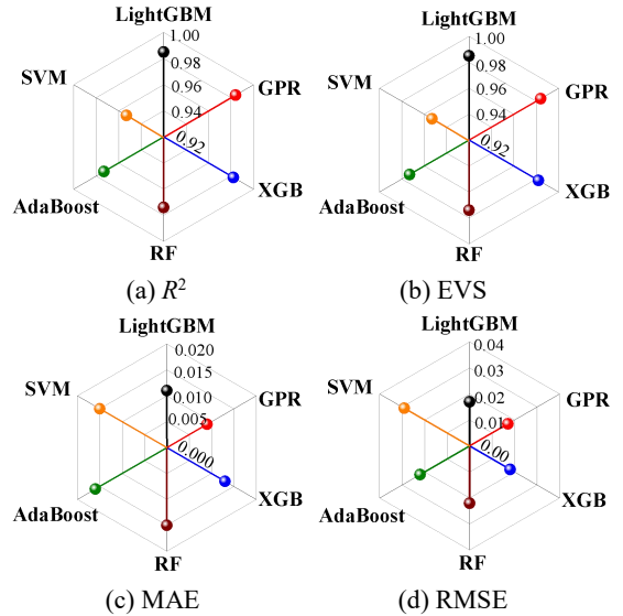
图 3 基于压力水头对数形式的机器学习算法性能评估 Fig.3 Performance evaluations of MLAs based on the logarithmic form of pressure head
