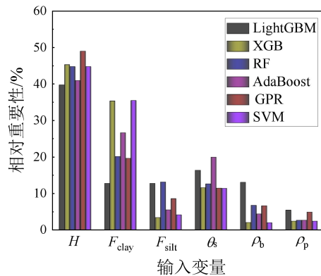
图 4 基于压力水头对数形式的输入变量特征重要性分析 Fig.4 Feature importance analysis of input variables based on logarithmic form of pressure head
